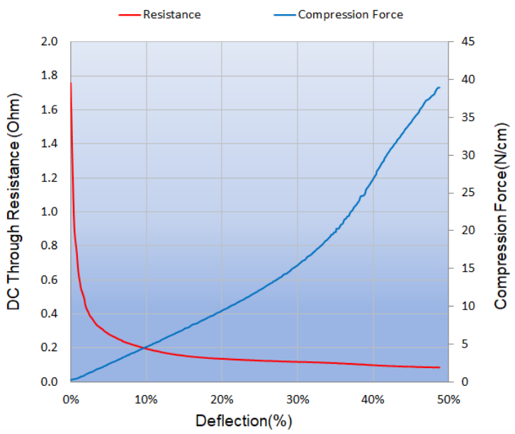
Force-Deflection-Resistance of F9304 Gasket 1.00mm (H) X 1.30mm (W) X 5.00mm (L)
