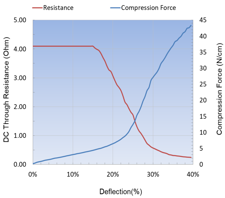
Force-Deflection-Resistance Curve of F5381 Gasket 1.0mm (H) X 1.25mm (W) X 5.00mm (L)
